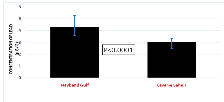
Figure 6: Comparison of lead in sediment in the Nayband Bay area (contaminated area) and Lavar-e Saheli (control area)
