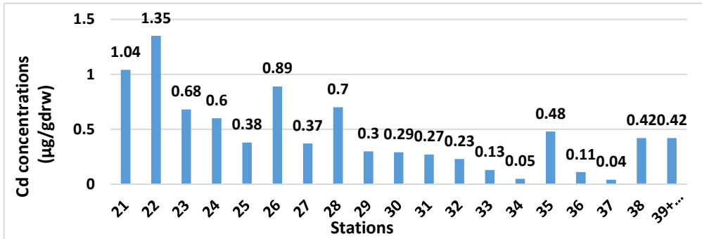
Figure 4: The concentration of cadmium in the sediments of the Lavar-e Saheli stations
