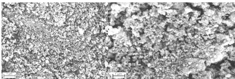
(a) (b) Fig. 2. SEM images of Fe 3 O 4 nanoparticles (a) and nanoparticles coated with alumina (b)
